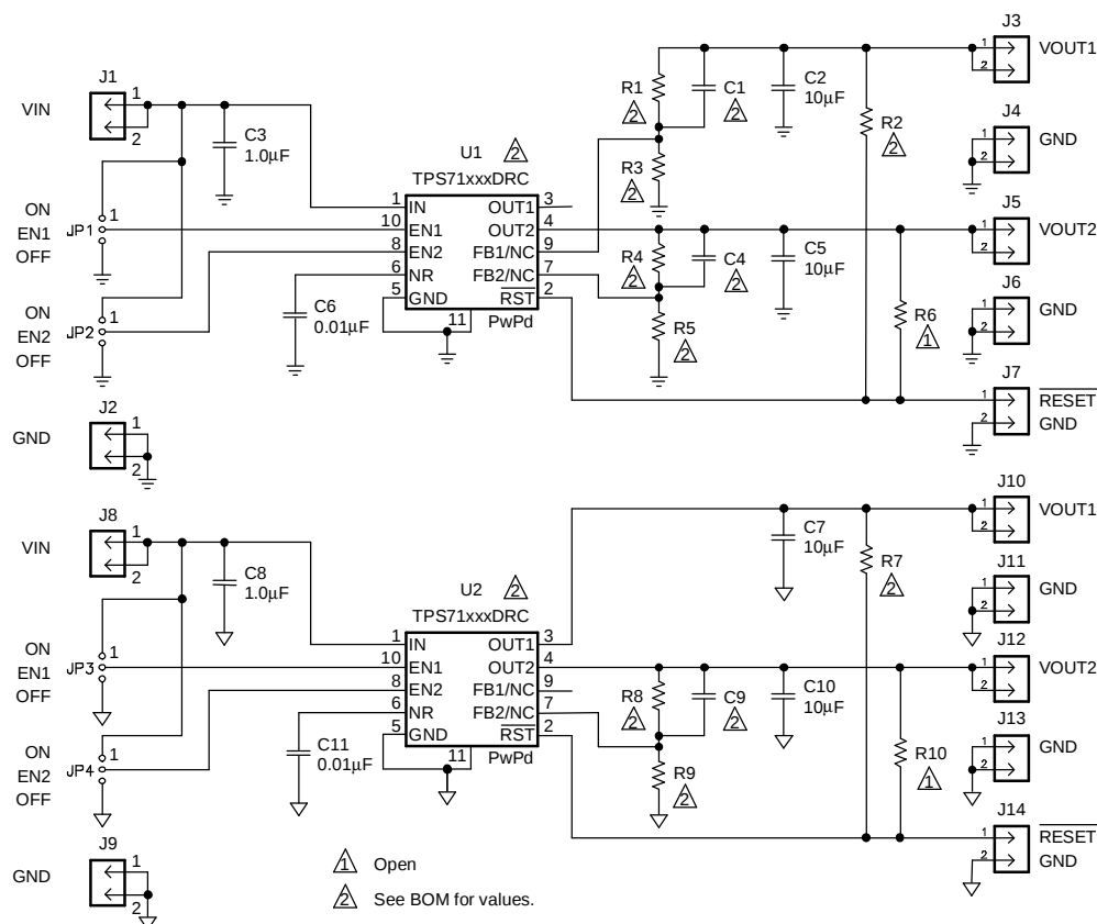
Figure 4. TPS713xxEVM-050 Schematic
